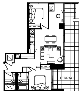
FLOOR 9
